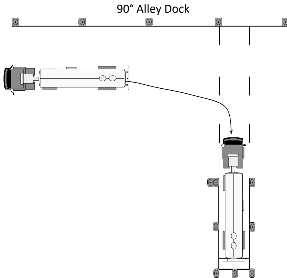
Figure 12.3: Alley Dock - 90°
