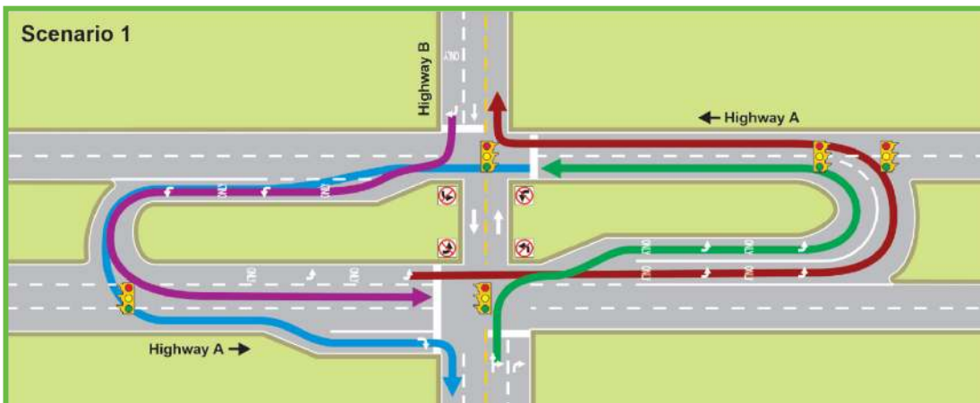
Figure 5.8. When drivers are prohibited from making a left turn at an intersection, they must circumvent the intersection and use the appropriate median crossover to complete their turn. (MDOT "Michigan Lefts," brochure - 9/23)
