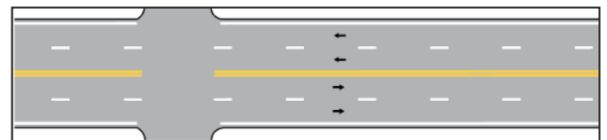
Figure 5.1 (FHWA/MUTCD: Figure 3B-2 (A), pg. 541)
