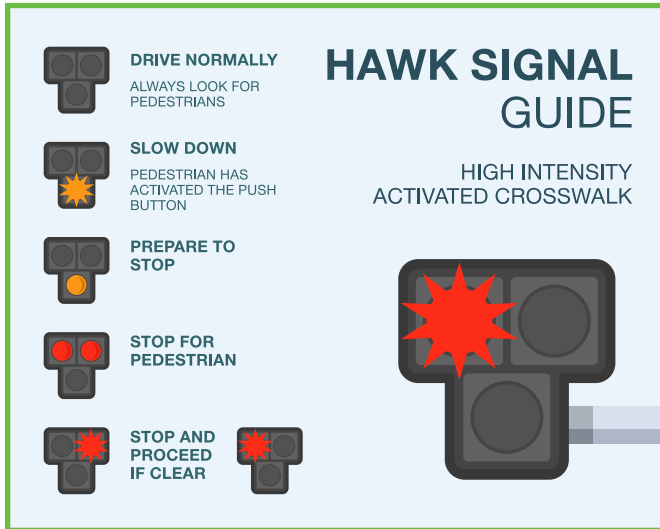
Figure 5.12. The Pedestrian Hybrid Beacon.
