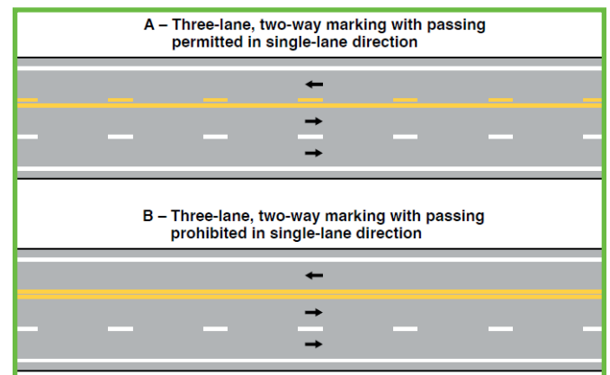
Figure 5.6. (FHWA/MUTCD: Figure 3B-3, pg. 542)
