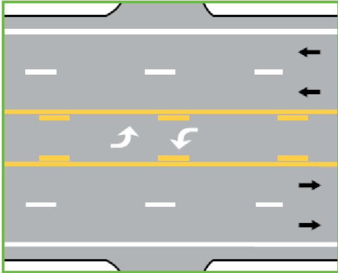
Figure 5.7. Left turns must be made from within the left-turn-only center lane and may be made from either direction. Using this lane to pass other vehicles or as a merge lane is illegal and dangerous. (FHWA/MUTCD Figure 3B-7, pg. 547)
