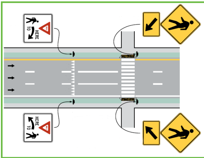
Figure 6.1. (FHWA/MUTCD, Figure 3B-16 (B), pg. 574)
