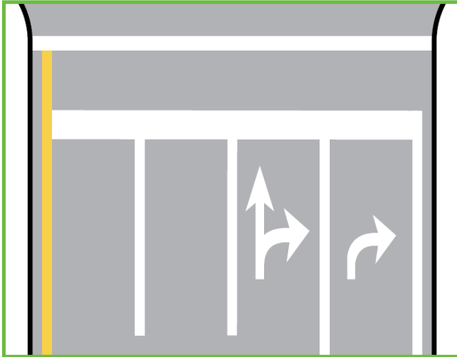
Figure 5.5 (FHWA/MUTCD: Figure 3B-13 B, pg. 564)
