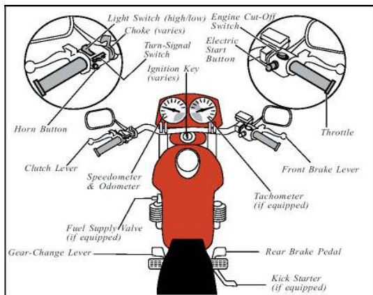
Motorcycle controls
