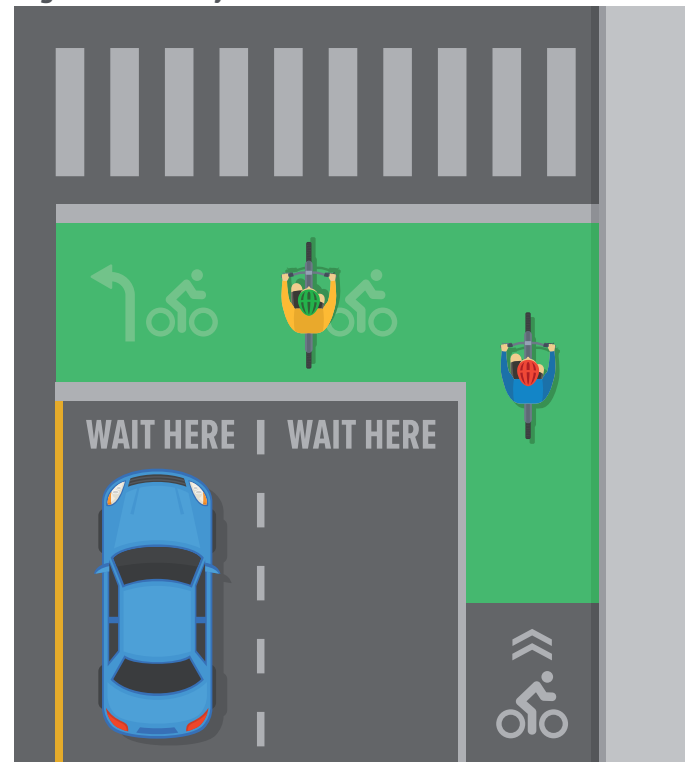
Figure 2.12: Bicycle boxes
